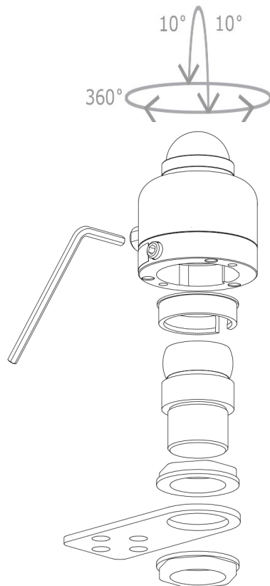
Figure 4.4.1 How to place 16103.5 on the ball levelling mounting set
