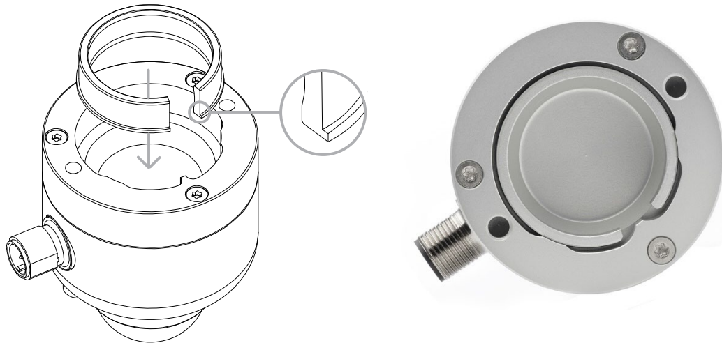
Figure 4.5.1 Line drawing indicating placement of the aluminum shim and photo showing the shim properly positioned in the centre of 16103.5's bottom plate. Note the position of the protruding ledge when placing the shim.
