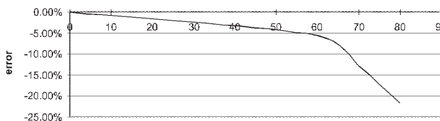
Fig. 3: The directional response or cosine response of the net radiometer 16123. On the horizontal axis the zenith angle (0° zenith angle equals 90° angle of incidence). On the vertical axis the percentage deviation from ideal cosine behavior. The specifications of the net radiometer regarding the cosine response are very good because the detector surface is shaped like a cone.
