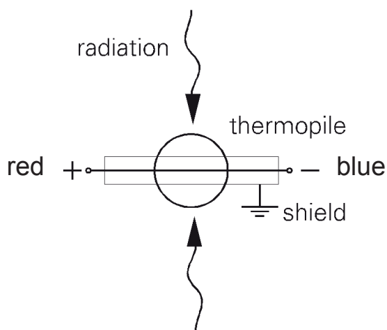
Fig. 1: Electrical circuit of the net radiometer
