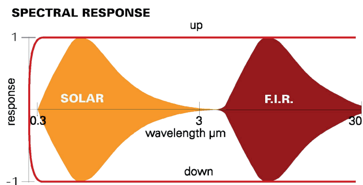
Fig. 2: The approximate spectral sensitivity of the net radiometer 16123 combined with the spectrum of the sun under a clear sky, and the spectrum of outgoing far infrared radiation.
